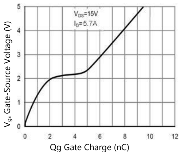
Figure 11. Gate Charge
