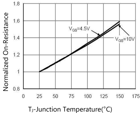
Figure 8. R_{dson} vs Junction Temperature
