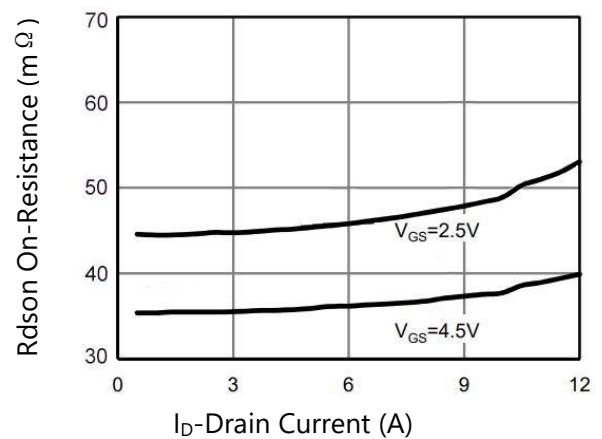
Figure 6. Drain-Source On-Resistance
