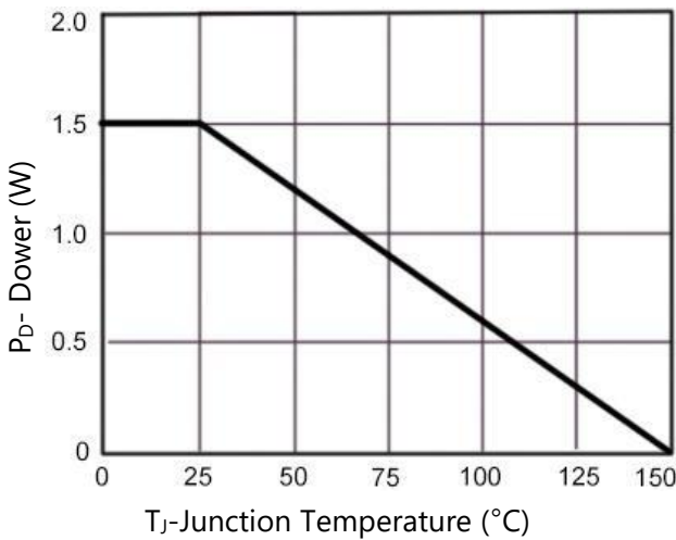
Figure 3. Power De-rating
