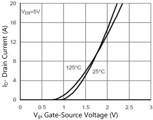
Figure 7. Transfer Characteristics
