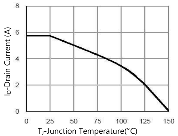
Figure 4. Drain Current
