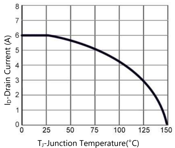
Figure 4. Drain Current
