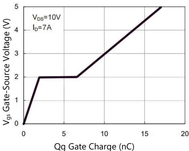
Figure 11. Gate Charge
