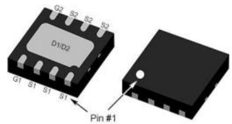
DFN3X3-8L top & bottom view
