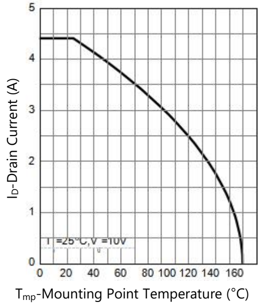
Figure 2. Current Capability
