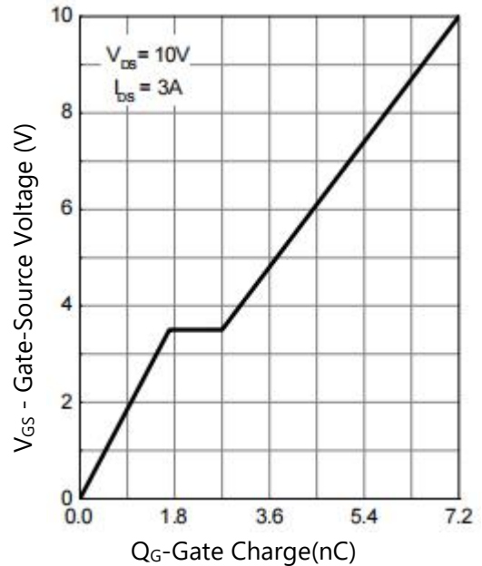
Figure 12. Gate Charge
