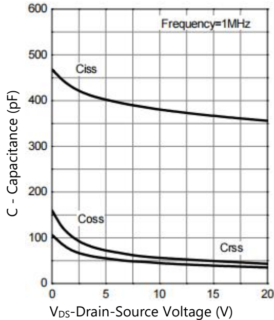
Figure 11. Capacitance
