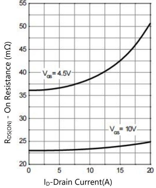
Figure 6. On Resistance
