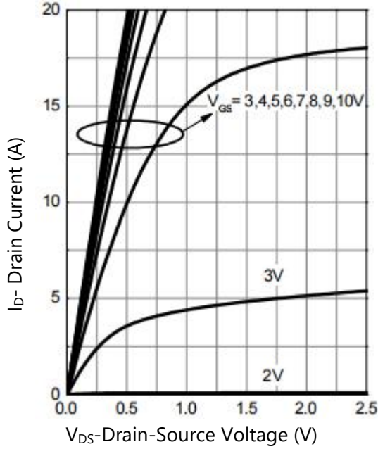
Figure 5. Output Characteristics
