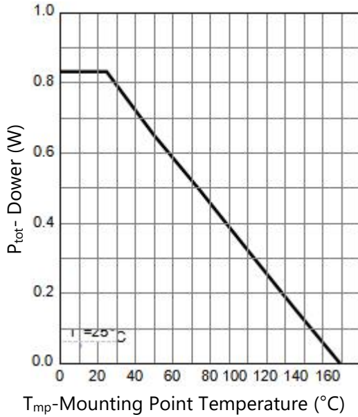
Figure 1. Power Capability
