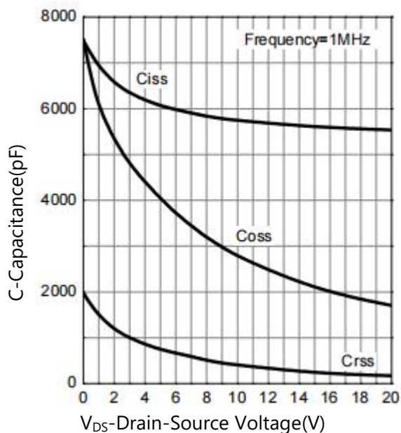
Figure 11. Capacitance
