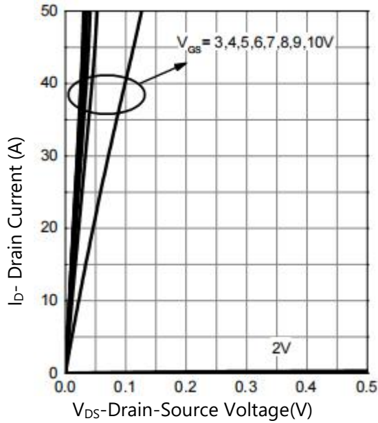
Figure 5. Output Characteristics
