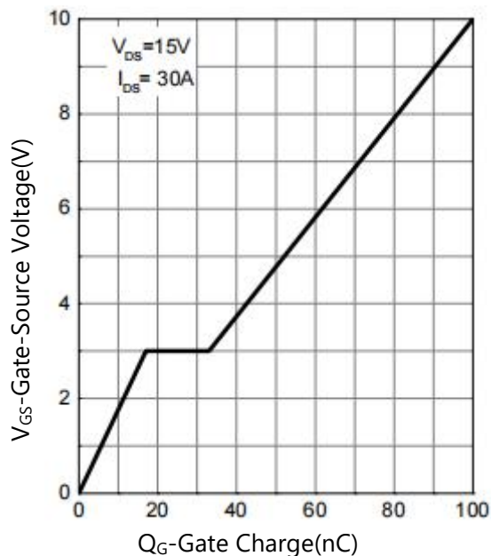
Figure 12. Gate Charge
