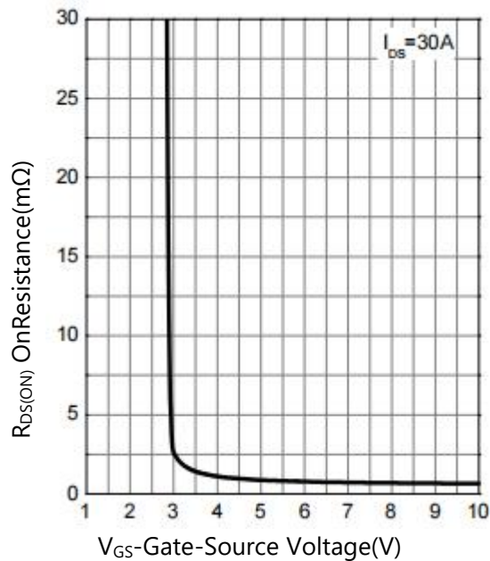
Figure 7. Transfer Characteristics
