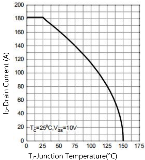
Figure 2. Current Capability
