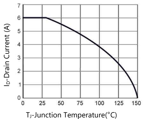
Figure 4. Drain Current
