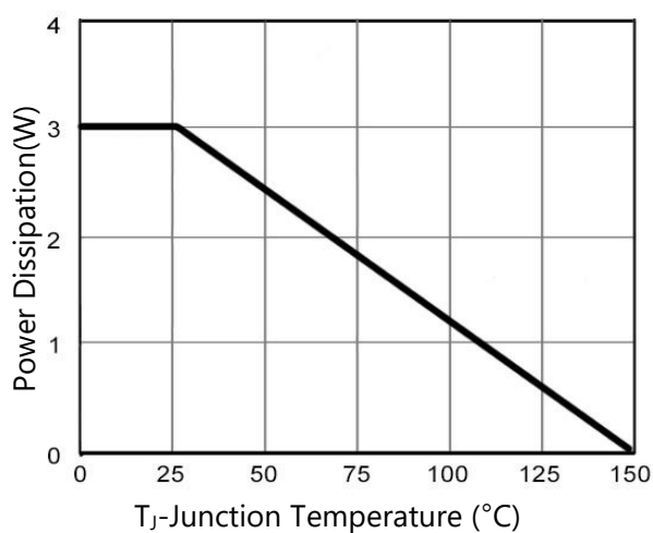
Figure 3. Power Dissipation
